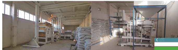
5T/H Green Mung Bean Cleaning Plant in Uzbekistan
