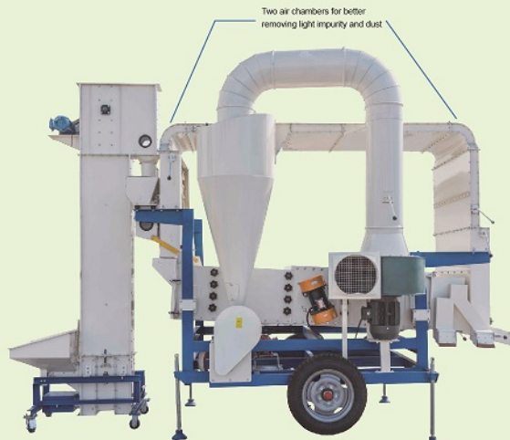
5XZC-7.5DS Seed Cleaner & Grader (double air cleaning system)
