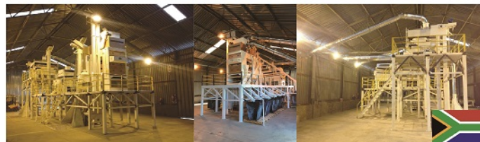
10T/H Sugar Bean Seed Processing Plant in South Africa
