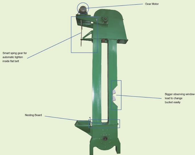
DTY-S Bucket Elevator (very low damage rate)
